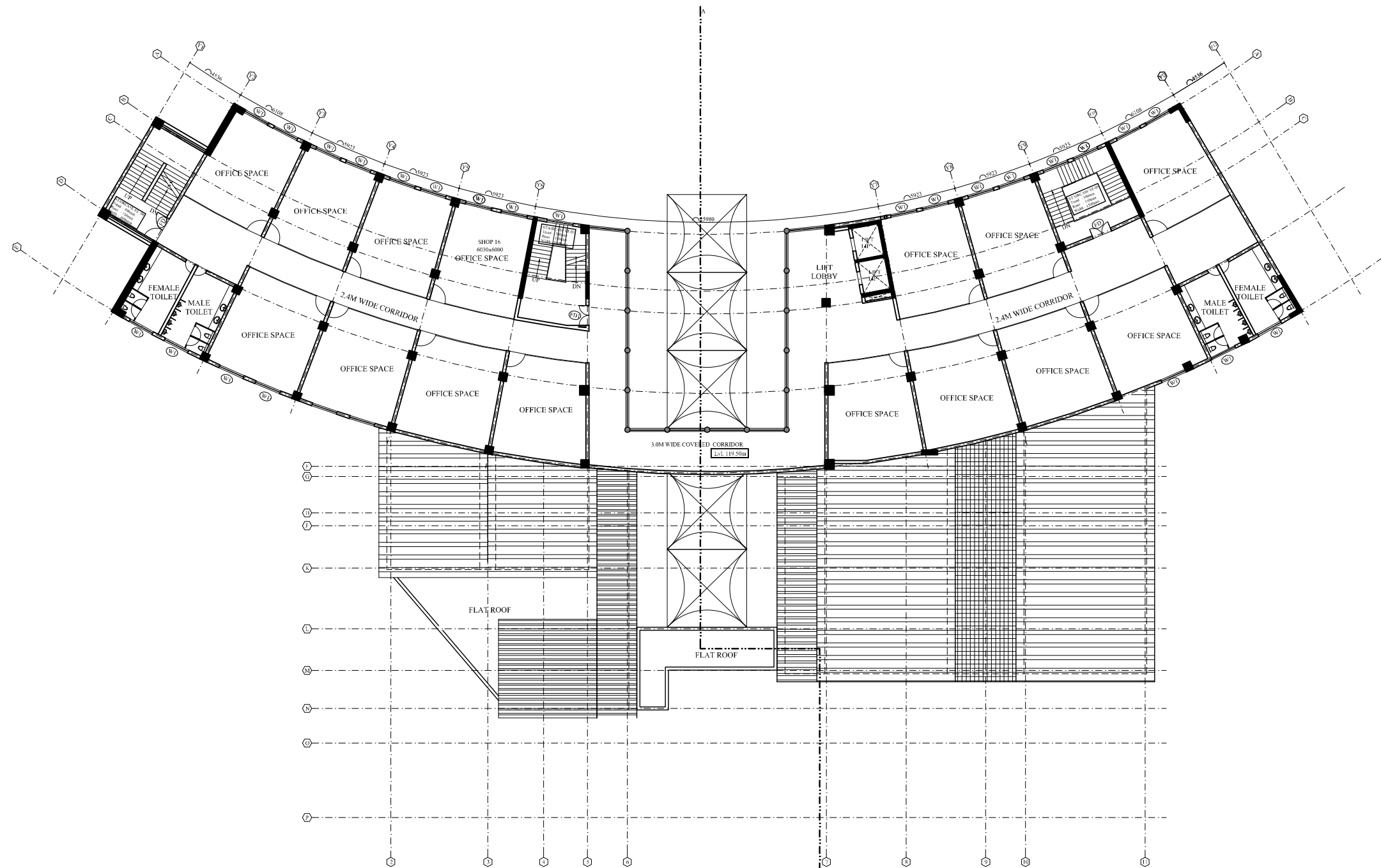
FOURTH FLOOR PLAN
